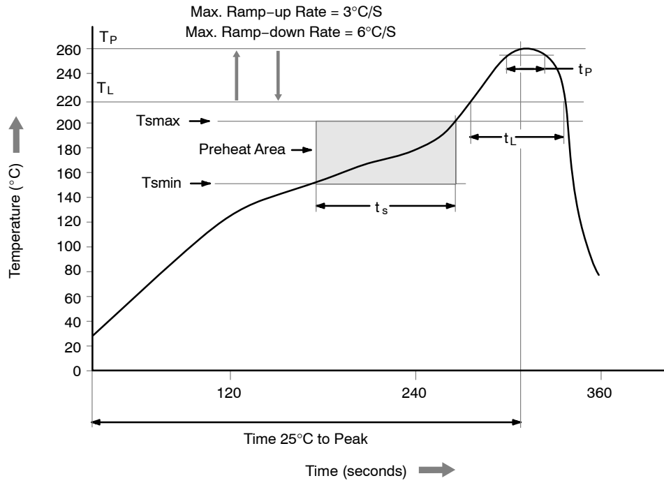
Figure 31. Reflow Profile
