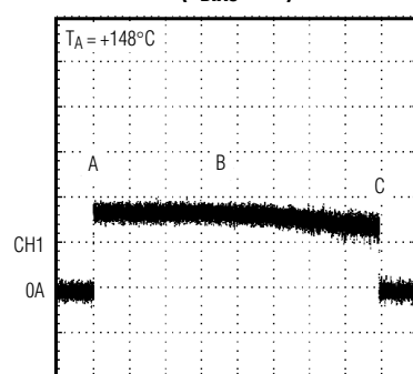
SHORT-CIRCUIT RESPONSE ( V_{\text{BIAS}} = 5\text{V} )
