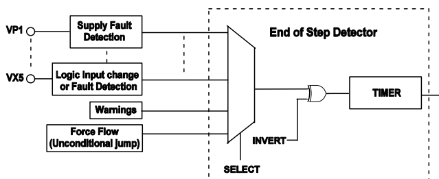
Figure 30. End-of-Step Detector
