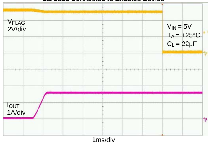
2Ω Load Connected to Enabled Device
