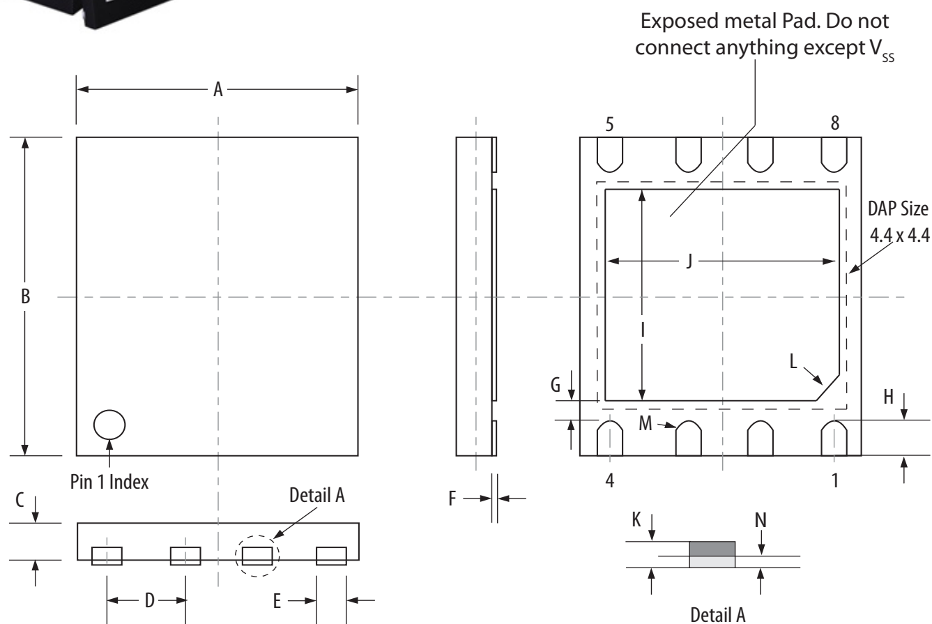
Figure 6.1 DFN Package
