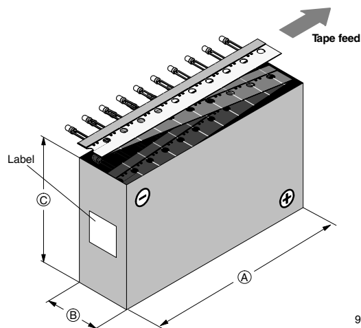
Fig. 20 - Tape Direction
