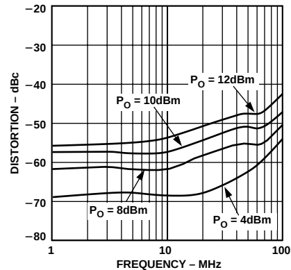
Figure 15. Worst Harmonic Distortion vs. Frequency for Various Output Levels at V_{CC} = 6V
