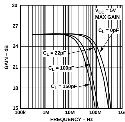
Figure 27. AC Response for Various Capacitive Loads
