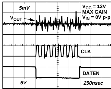
Figure 32. Clock Feedthrough Glitch
