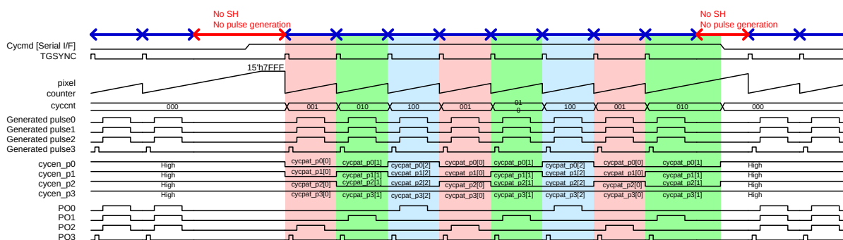
Figure 23 TG Cycle Mode
