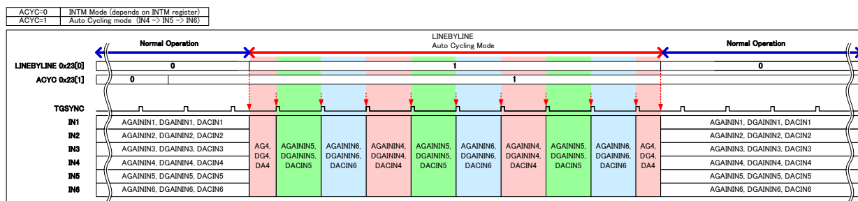
Figure 31 Line-by-Line Operation (ACYC=1, Auto-cycling mode)
