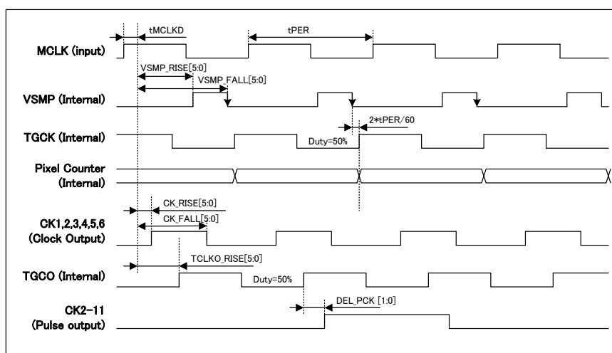
Figure 18 TG Output Timing
