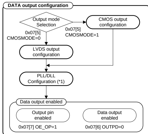
Figure 47 Data Output Configuration
