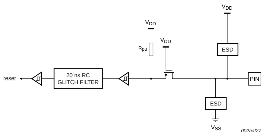
Fig 52. Reset pad configuration
