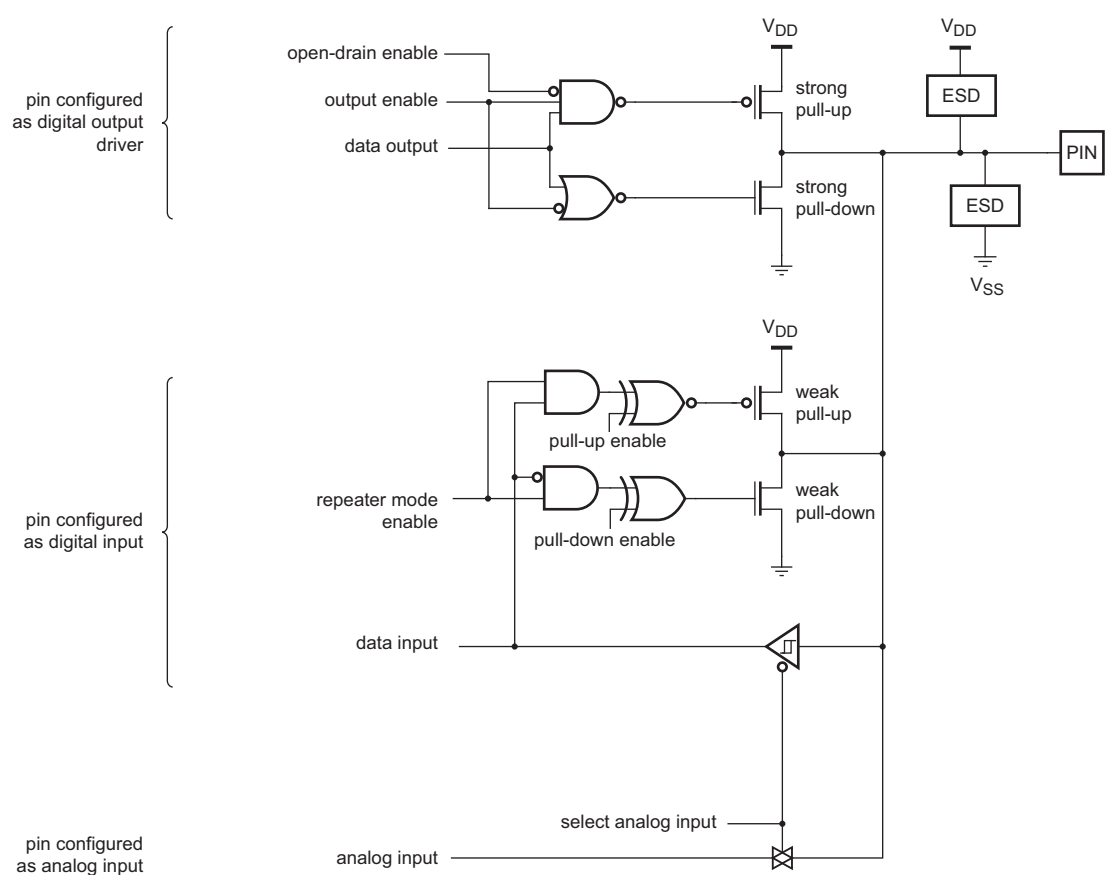
Fig 51. Standard I/O pad configuration
