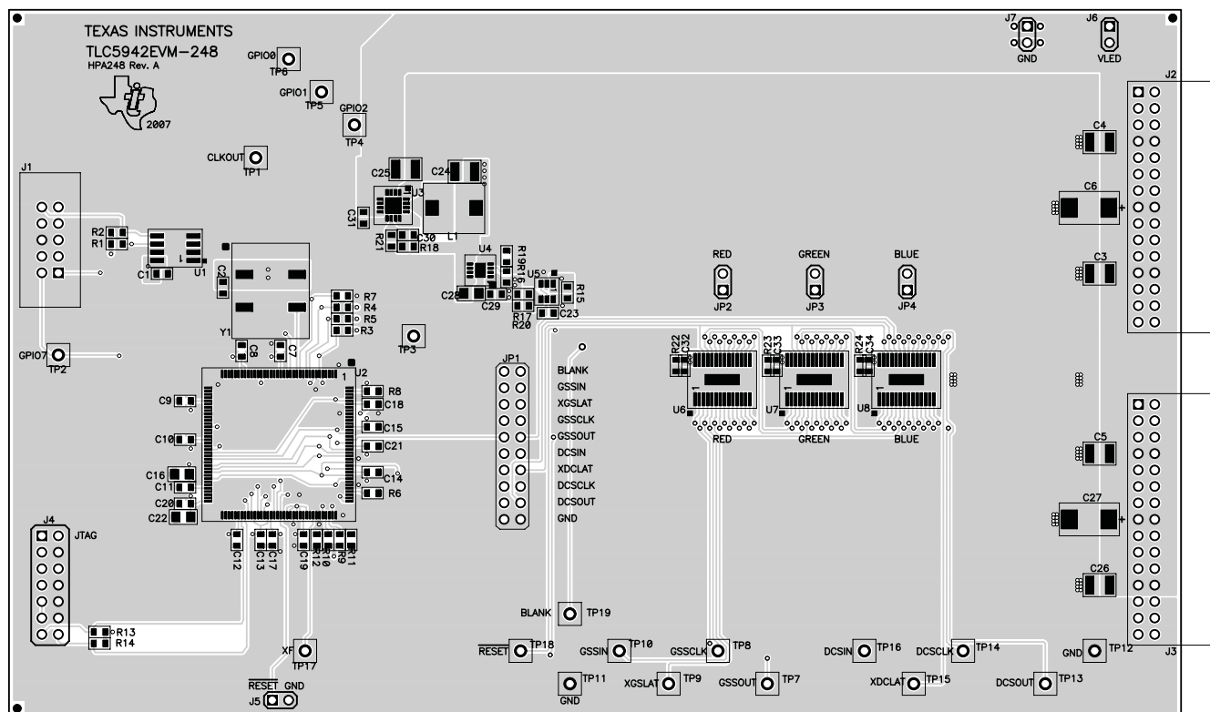
Figure 6. Assembly Layer
