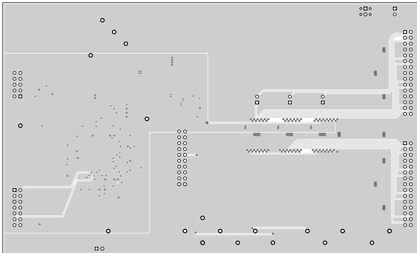
Figure 9. Layer 3
