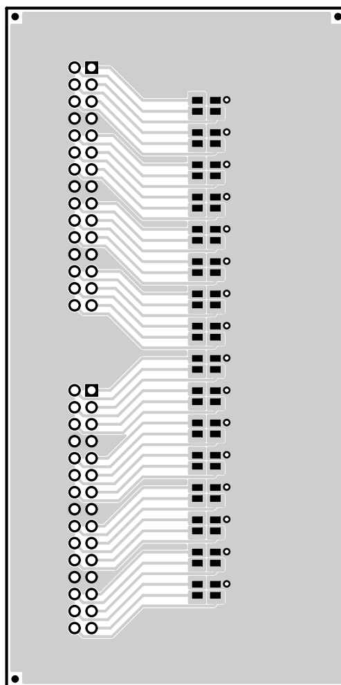
Figure 12. Top Layer
