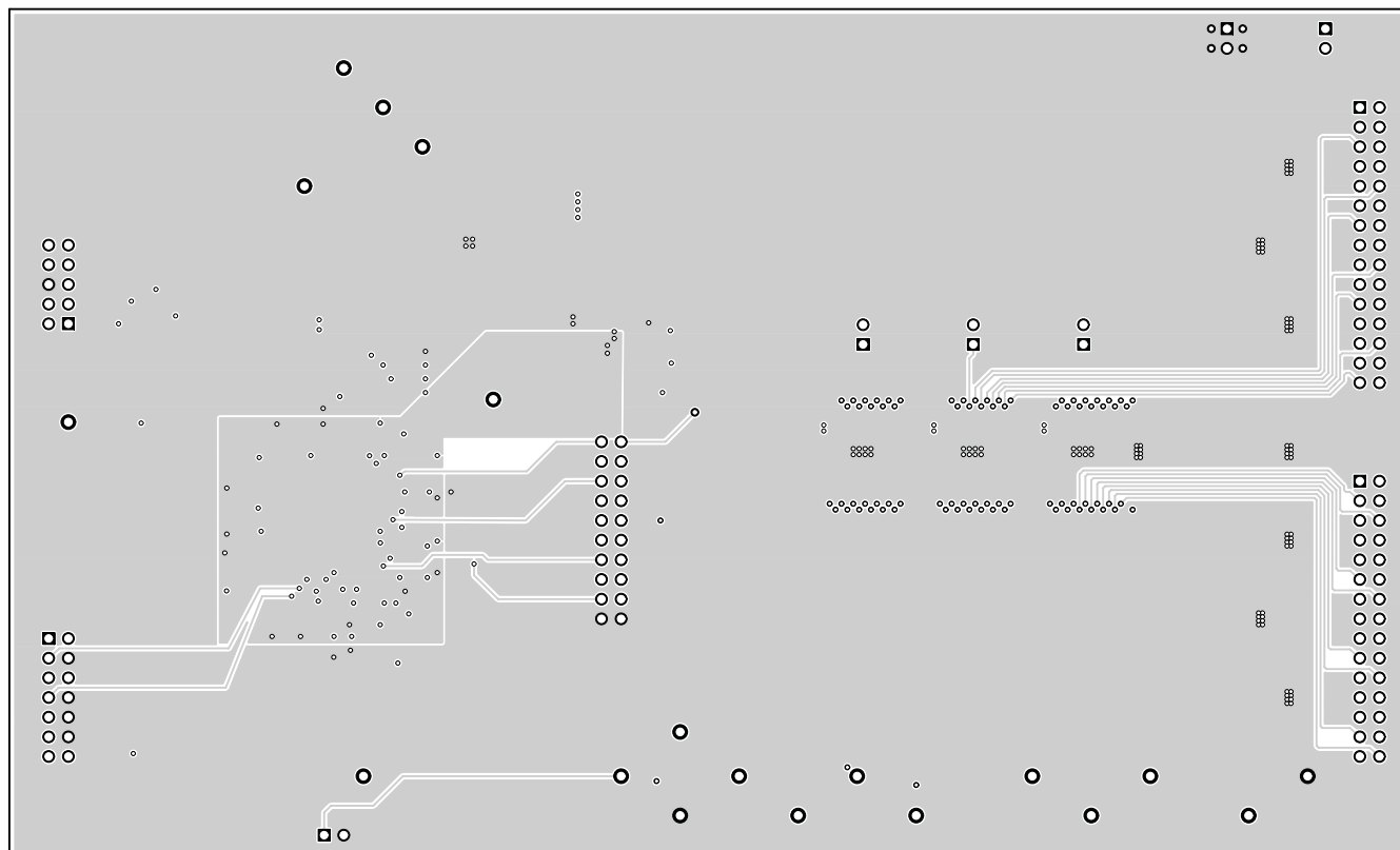
Figure 8. Layer 2
