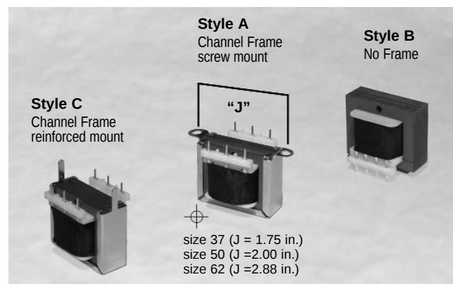
PC Series (concentric) is shown; primary 47/500 Hz; EL Series (split bobbin) available; primary 50/60 Hz.
