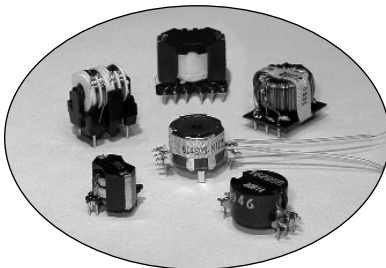
Thru-hole pc-mount, surface-mount, low-profile, vertical and horizontal, chassis mount.
