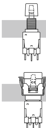
Bushing Mount
