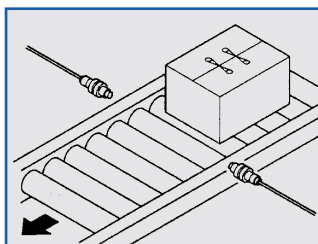
Object detection
