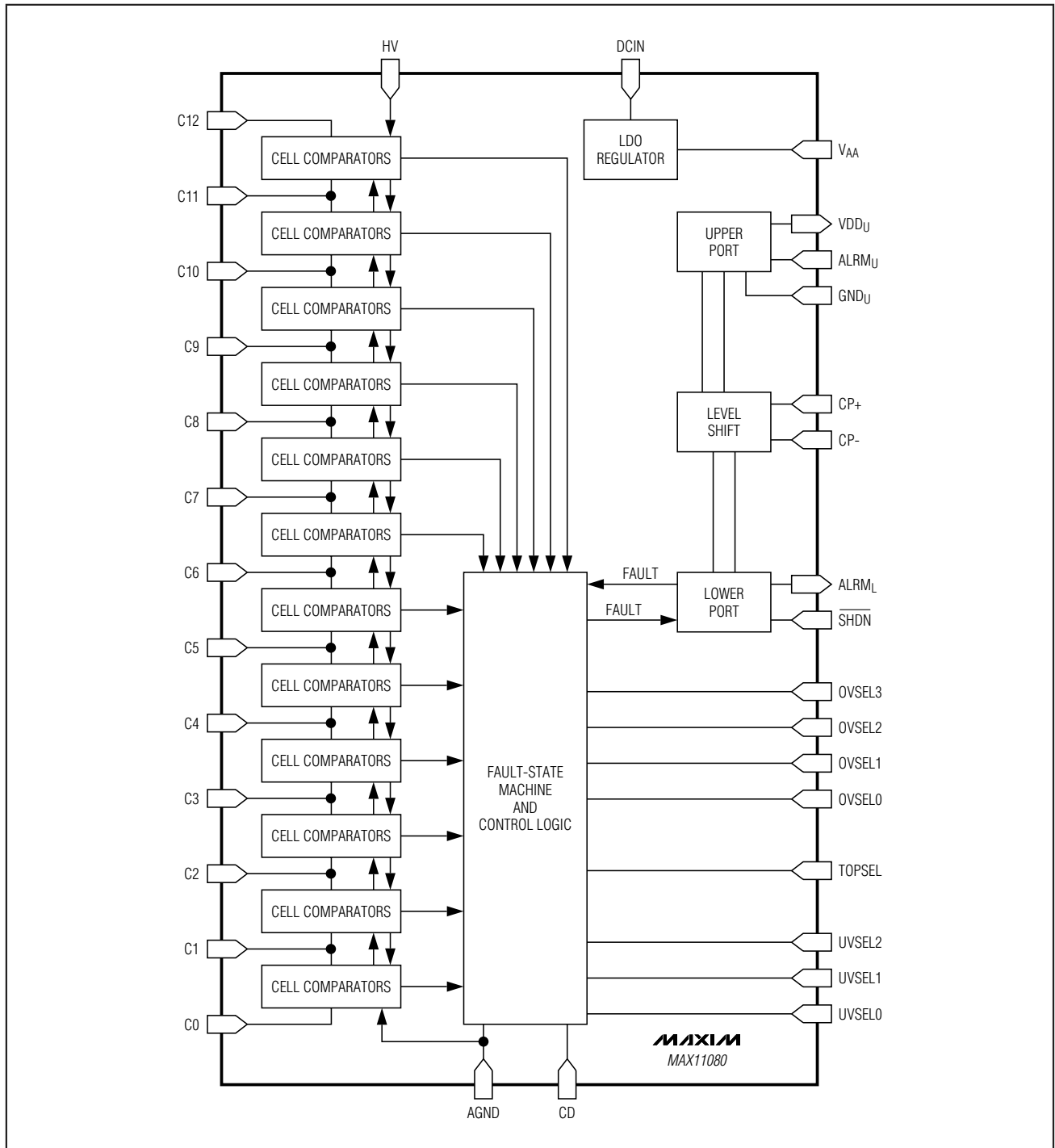
Figure 1. Functional Diagram
