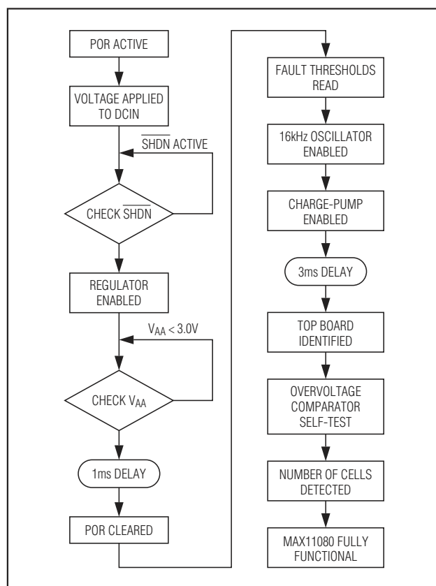
Figure 12. Linear Regulator Power-Up Sequence
