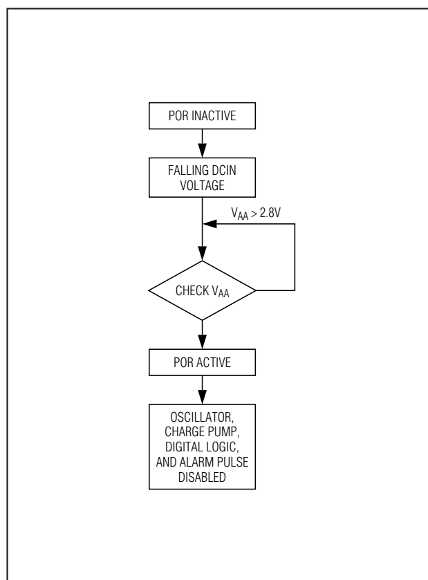
Figure 13. Low DCIN POR Event
