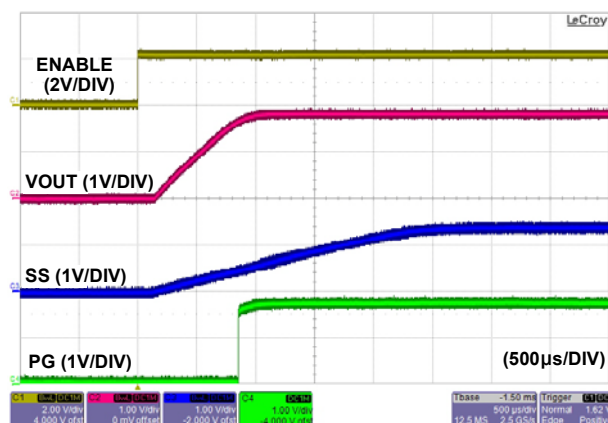
FIGURE 12. ENABLE START-UP ( C_{SS} = 2.2nF )
