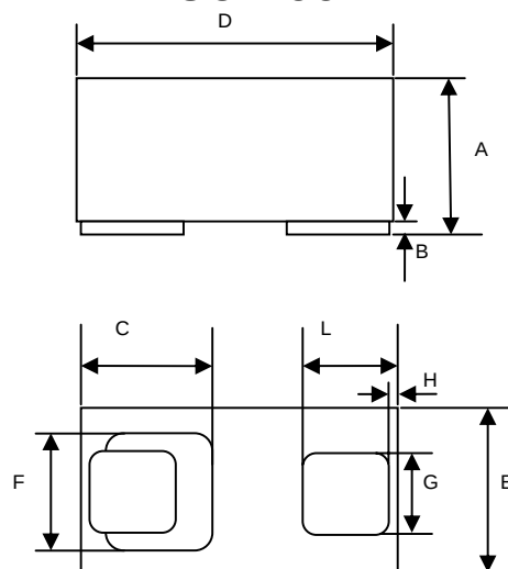
SOD-882
