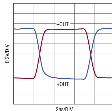
No-Overshoot Step Response
