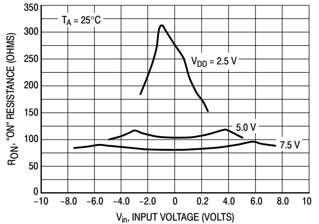
Figure 15. Comparison at 25°C, V_{DD} = -V_{EE}
