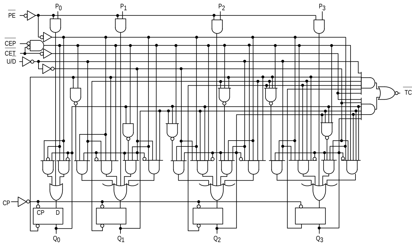
SN54/74LS169
