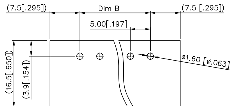
PCB LAYOUT
