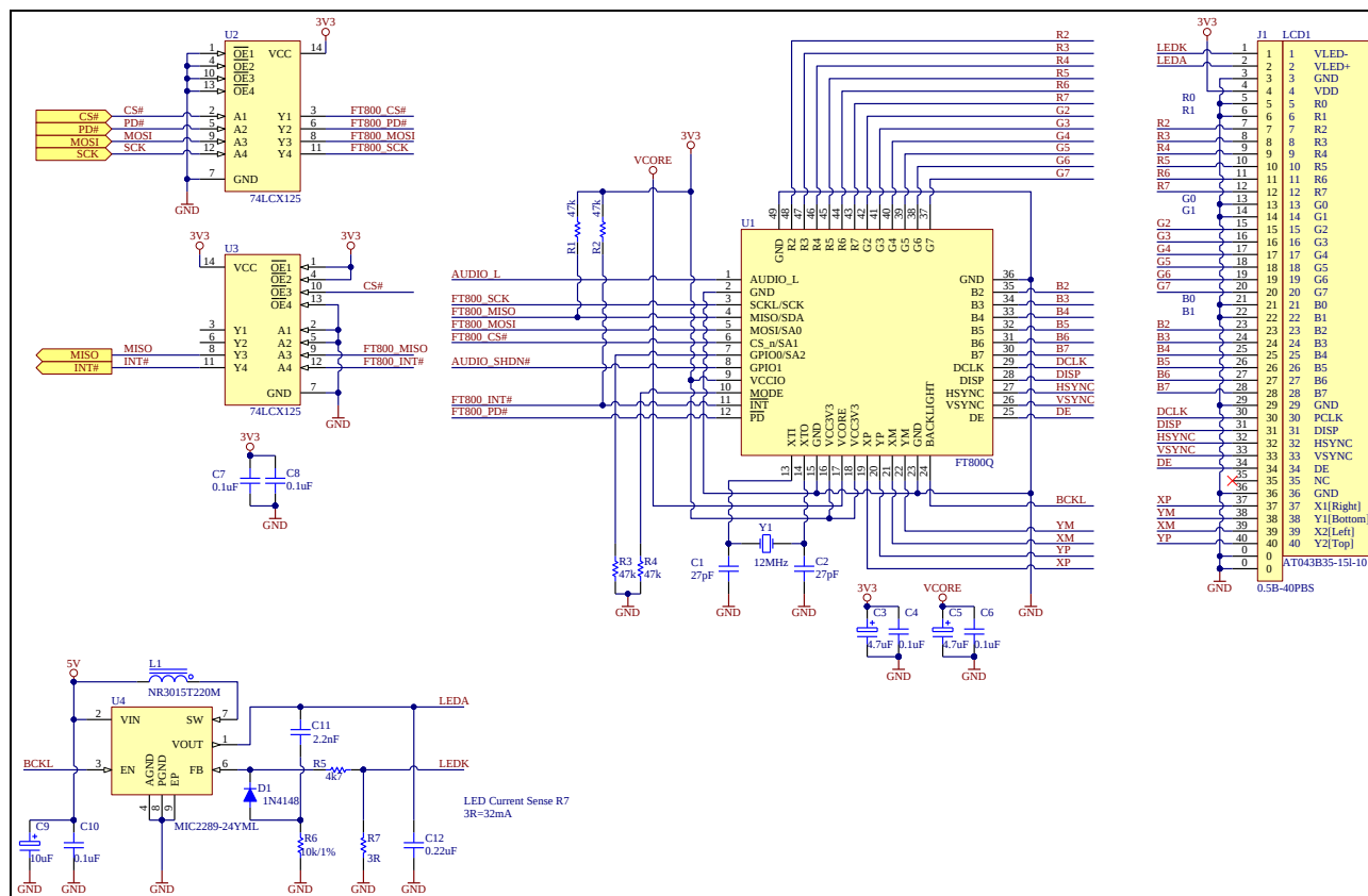
Figure 4-2 - VM800C43/VM800C50 (4.3"/5.0" Version)
