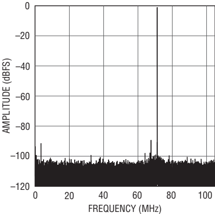
LTC2156-12: 32K Point FFT, f_{IN} = 71\text{MHz} , -1dBFS, 210Mpsps
