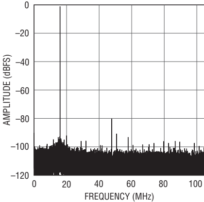
LTC2156-12: 32K Point FFT, f_{IN} = 227\text{MHz} , -1dBFS, 210Mpsps
