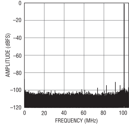
LTC2156-12: 32K Point FFT, f_{IN} = 101\text{MHz} , -1dBFS, 210Mpsps
