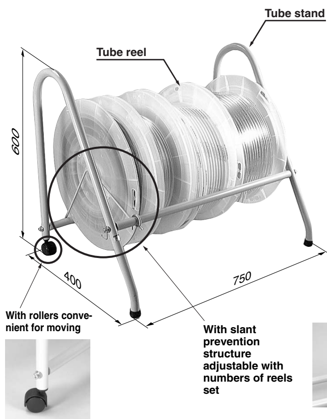
Tube Reel: TBR-1/2/3/4
