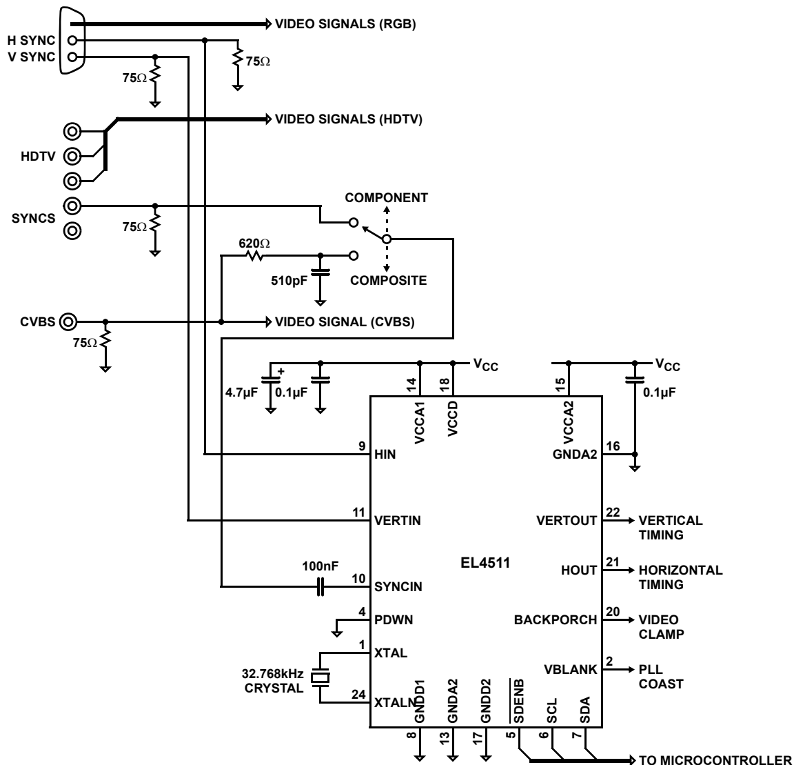
FIGURE 12. APPLICATIONS DRAWING 3
