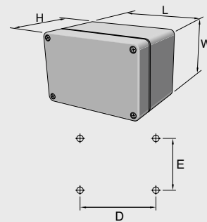
Montagemaß Mounting dimensions Montageafmetingen
