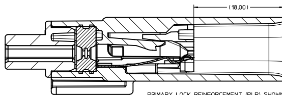
SECTION Y-Y
