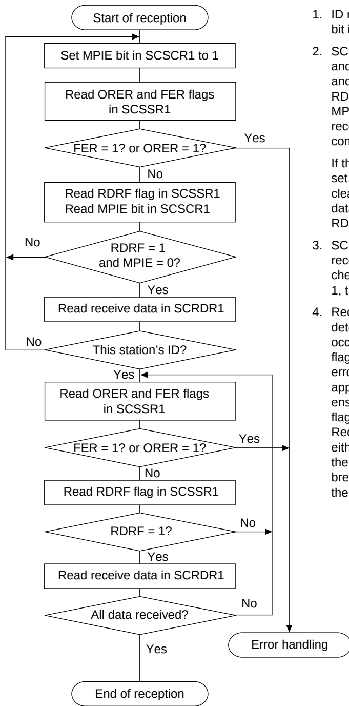
Figure 15.15 Sample Multiprocessor Serial Reception Flowchart (1)
