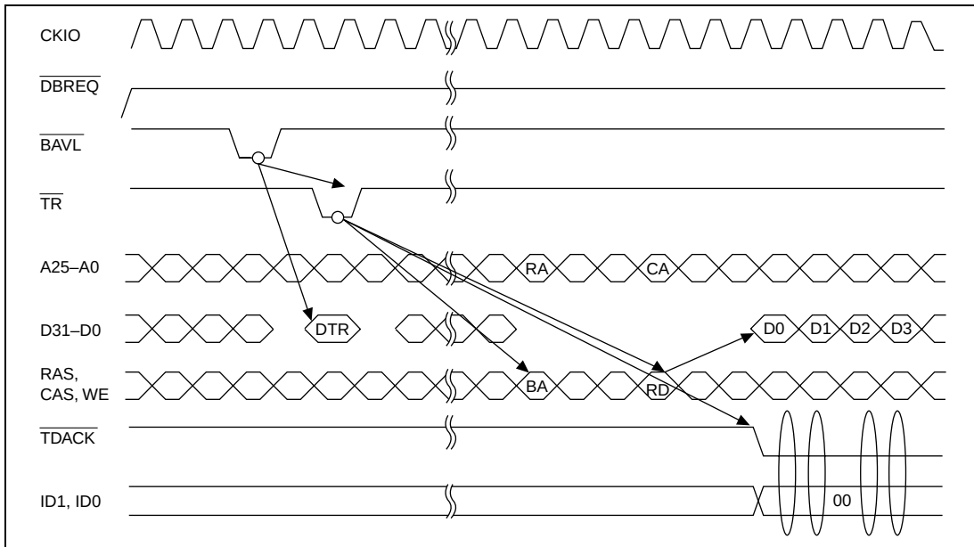
Figure 14.29 Single Address Mode/Burst Mode/External Device → External Device 32-Byte Block Transfer/Channel 0 On-Demand Data Transfer
