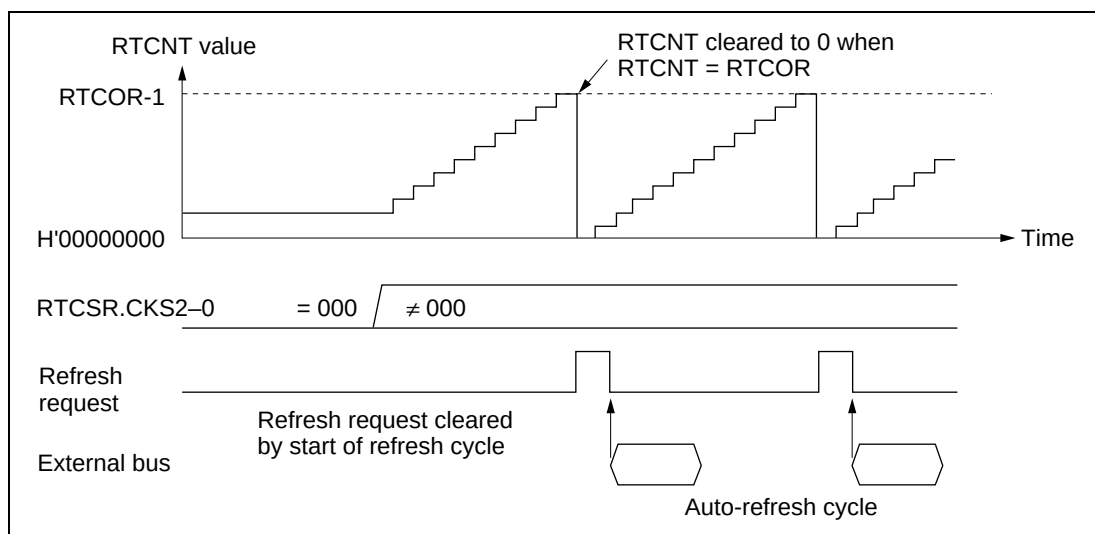
Figure 13.35 Auto-Refresh Operation
