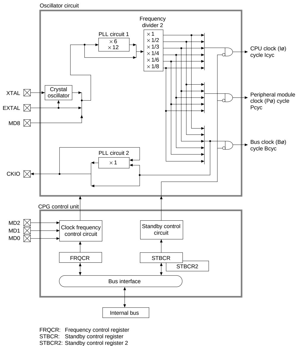
Figure 10.1(2) Block Diagram of CPG (SH7751R)
