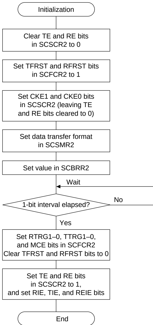
Figure 16.7 Sample SCIF Initialization Flowchart
