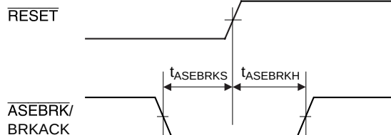
Figure 23.66 \overline{\text{RESET}} Hold Timing
