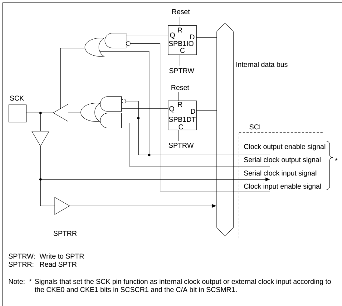
Figure 15.2 SCK Pin
