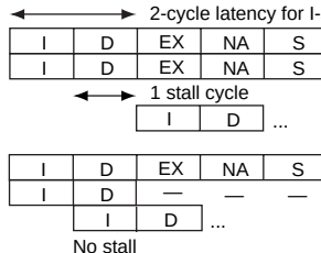
Figure 8.3 Examples of Pipelined Execution
