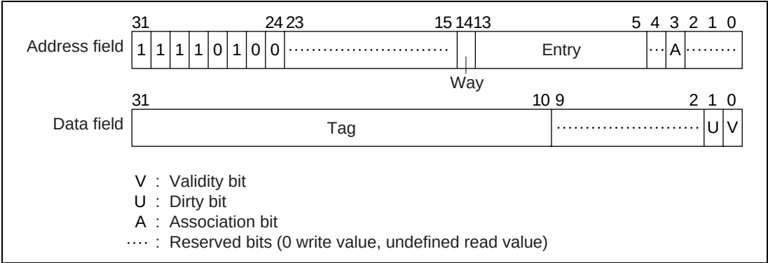
Figure 4.14 Memory-Mapped OC Address Array
