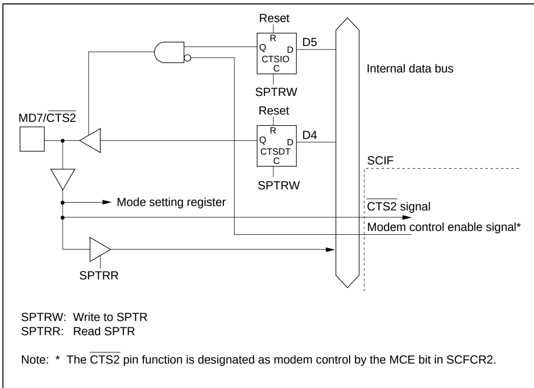
Figure 16.3 MD7/CTS2 Pin
