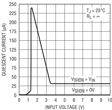
LT1763-3.3 Quiescent Current
