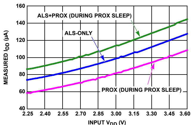
FIGURE 11. V_{DD} vs I_{DD} FOR VARIOUS MODES OF OPERATION
