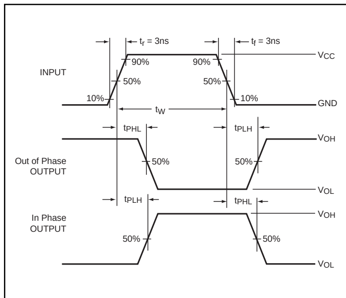
Figure 3. AC Waveforms
