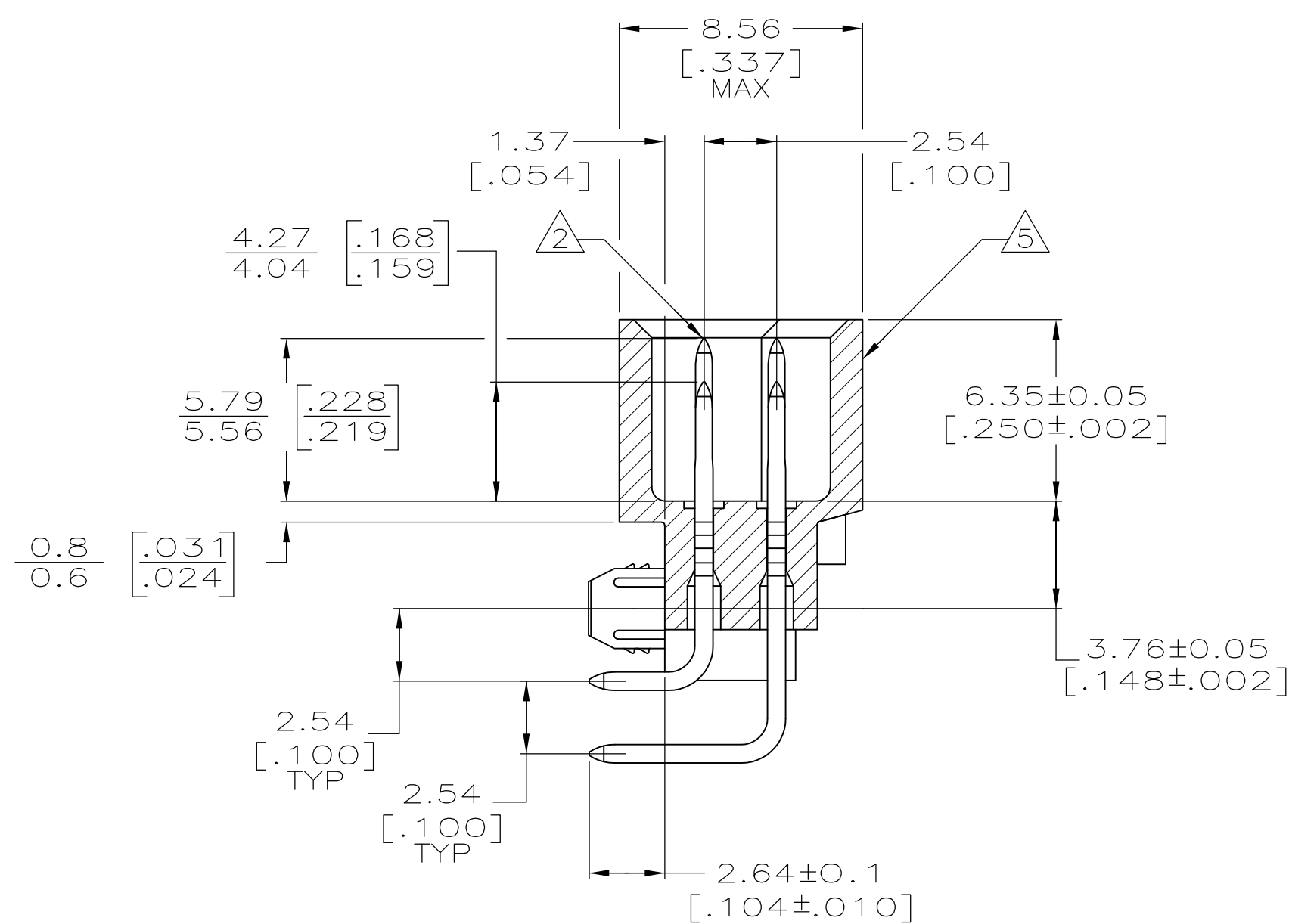
SECTION Z-Z
