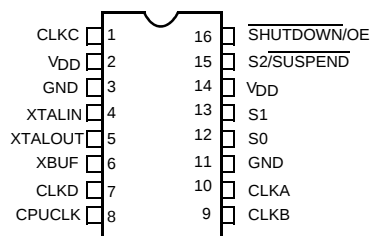
Figure 1. CY2292 – 16-pin SOIC
