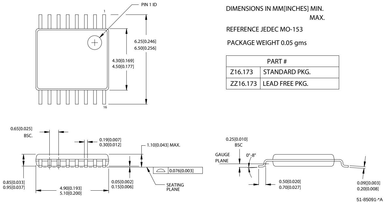
Figure 7. 16-Pin TSSOP 4.40 mm Body Z16.173
