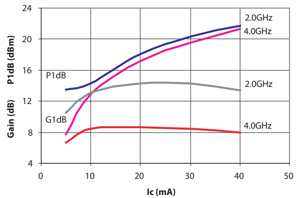
Figure 2. Output Power and 1dB Compression Gain vs. Collector Current and Frequency. V_{ce} = 8\text{V} .
