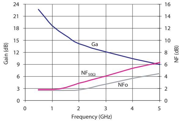
Figure 1. Noise Figure and Associated Gain vs. Frequency. V_{ce} = 8\text{V} , I_c = 10\text{mA}
