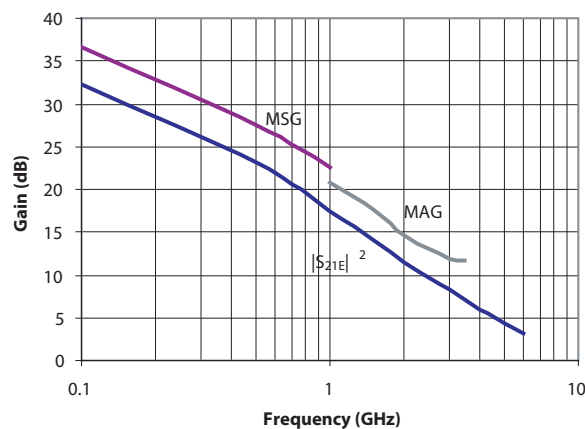
Figure 5. Insertion Power Gain, Maximum Available Gain and Maximum Stable Gain vs. Frequency. V_{ce} = 8\text{V} , I_c = 25\text{mA}
