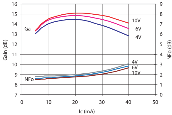
Figure 3. Optimum Noise Figure and Associated Gain vs. Collector Current and Collector Voltage. F = 2.0\text{GHz} .
