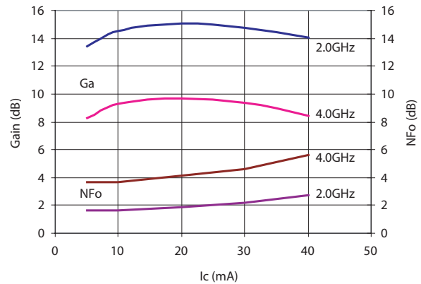
Figure 4. Optimum Noise Figure and Associated Gain vs. Collector Current and Frequency. V_{ce} = 8\text{V} .
