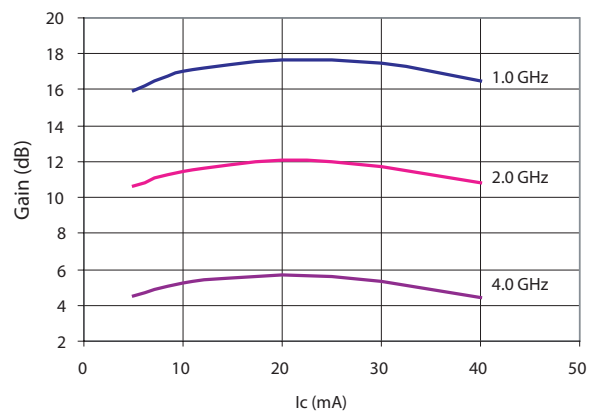
Figure 6. Insertion Power Gain vs. Collector Current and Frequency. V_{ce} = 8\text{V} .
