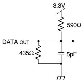
Figure 2. Output Test Load (For t HZ , t LZ , t WZ and t OW ) * Including scope and jig.
