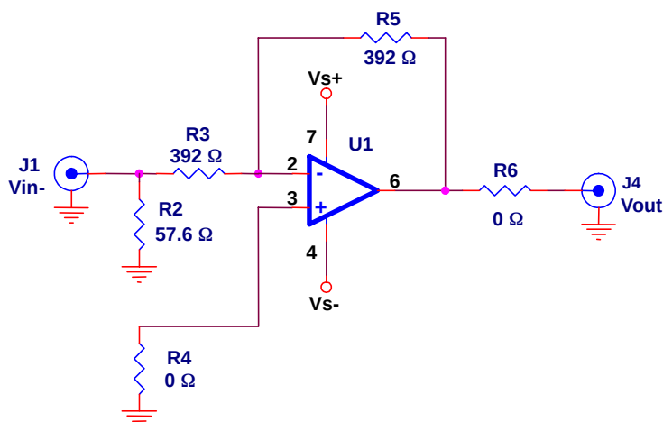
Figure 3-3. Inverting Gain Stage
