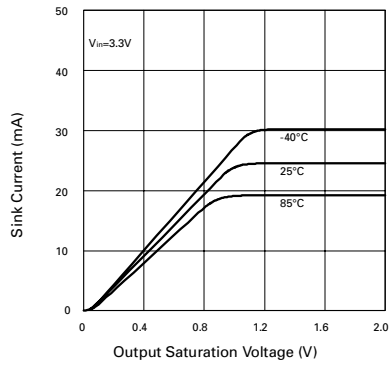
Output I(sink) vs. Output V(sat)
