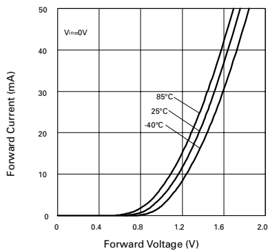
Clamp Diode I(forward) vs. Voltage
