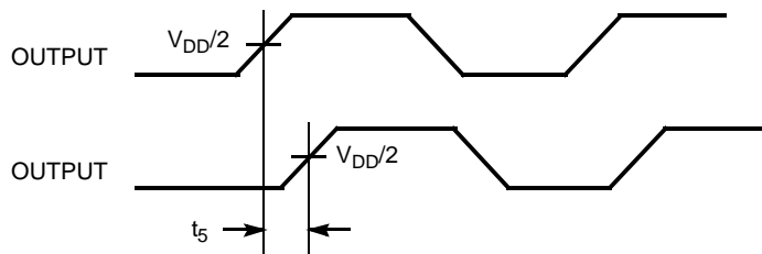
Output-Output Skew
