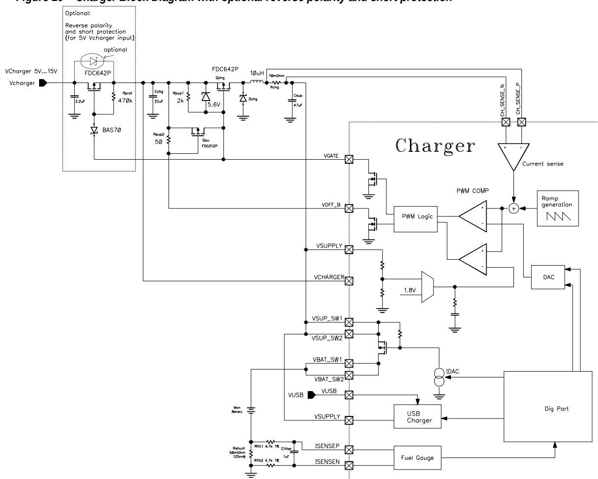
Figure 10 – Charger Block Diagram with optional reverse polarity and short protection
