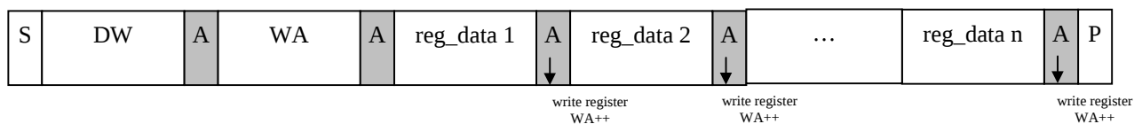
Figure 25 – I 2 C Page-Write:
