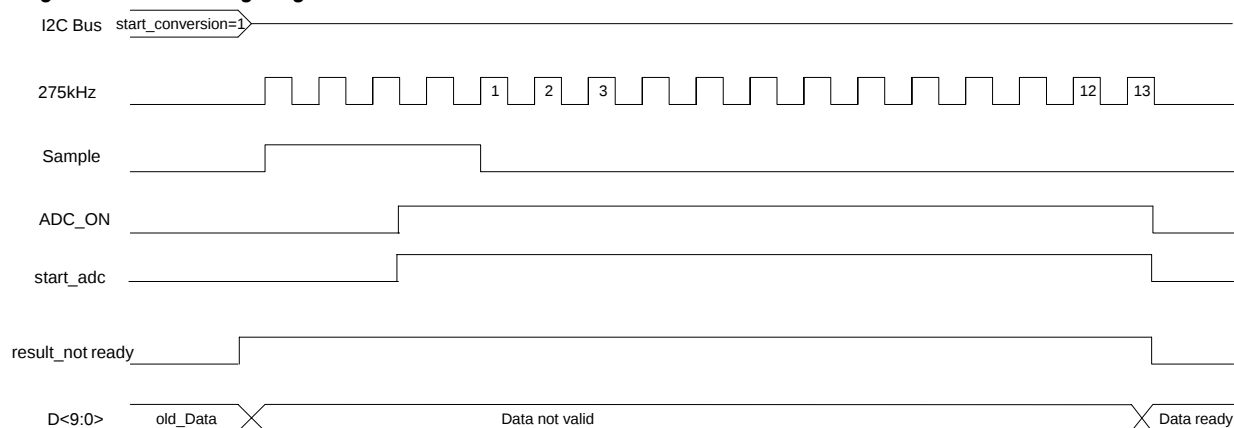
Figure 8 – ADC Timing-diagram
