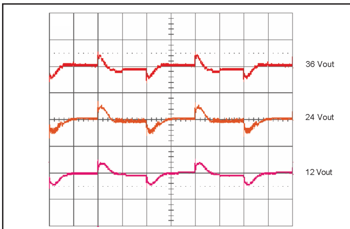
Figure 11: Output voltage response for 24V input; 12V, 24V, 36V output to step-change in load current (50-75-50% of Iout max; di/dt=0.1A/μs). Load cap: 100μF, 100mΩ ESR tant, Ch 1-3: Vout (2V/div);(5ms/div).
