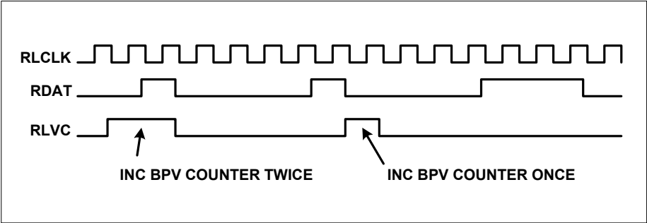
Figure 8-6. RX Line IO UNI Functional Timing Diagram
