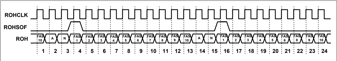
Figure 8-7. DS3 Framing Receive Overhead Port Timing
