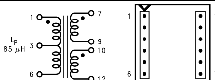
Figure 40. Renco RL-5534 (Top View)
