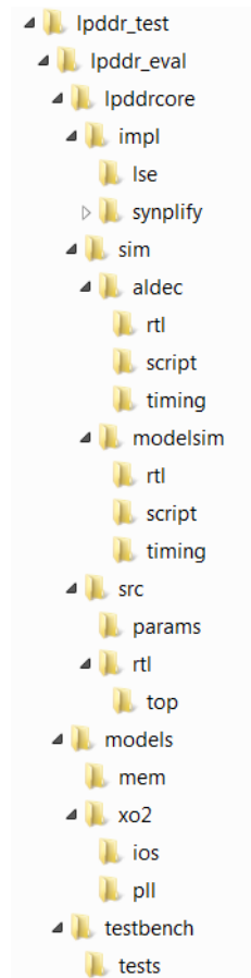
Figure 4-3. MachXO2 LPDDR Core Directory Structure
