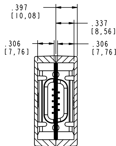
SECTION B-B
