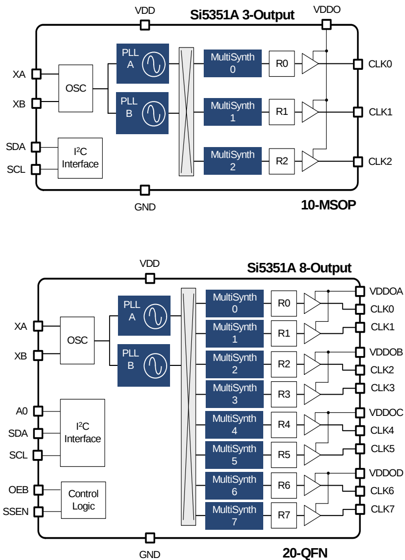
Figure 1. Block Diagrams of 3-Output and 8-Output Si5351A Devices
