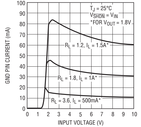
LT1963A-1.8 GND Pin Current
