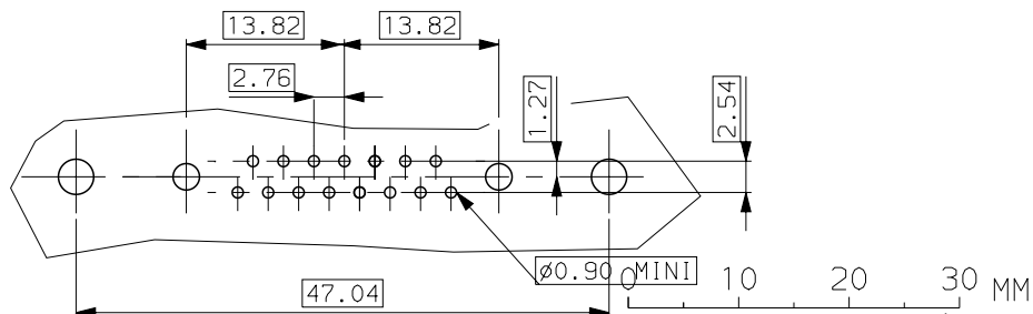
LAYOUT DIMENSIONS (after plating) CONNECTOR SIDE VIEW
