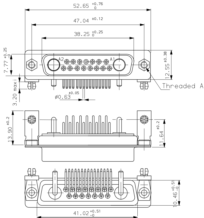
LAYOUT DIMENSIONS (after plating) CONNECTOR SIDE VIEW
