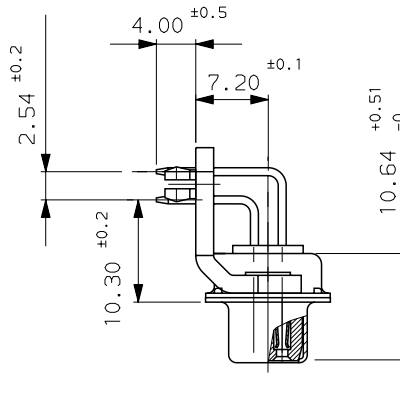
VIEW WITHOUT POWERS CONTACTS
