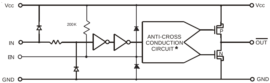
Figure 2 - IXDE509 Inverting 9A Gate Driver Functional Block Diagram
