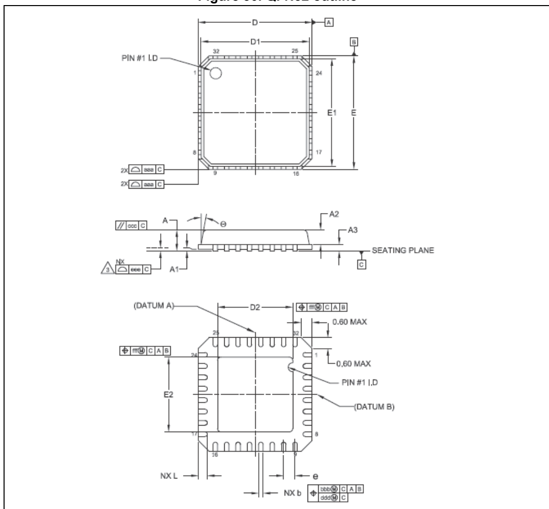
Figure 30. QFN32 outline
