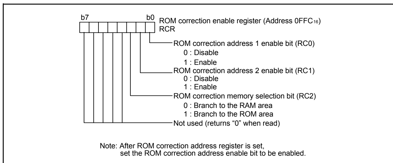
Fig. 50 Structure of ROM correction enable register
