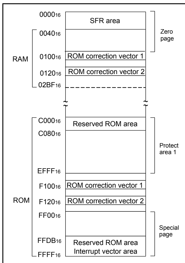
Fig. 49 Memory map of M38D24G4
