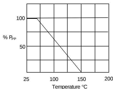
Figure 4 - Derating Curve
